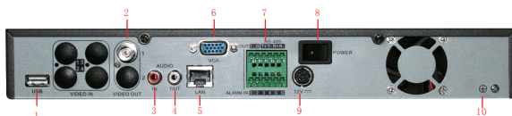
Rear Panel of DS-7604 NI-S
